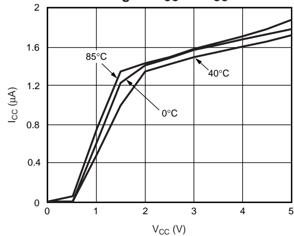
Fig. 7 – I_{CC} vs. V_{CC}
